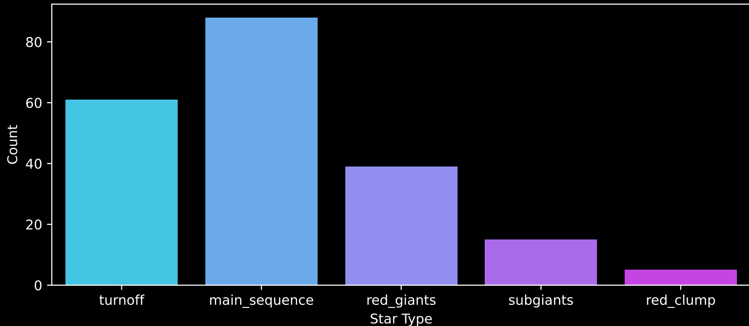
APOGEE DR17 Field: [K2_C3_043-50] Count plot of Star Type
