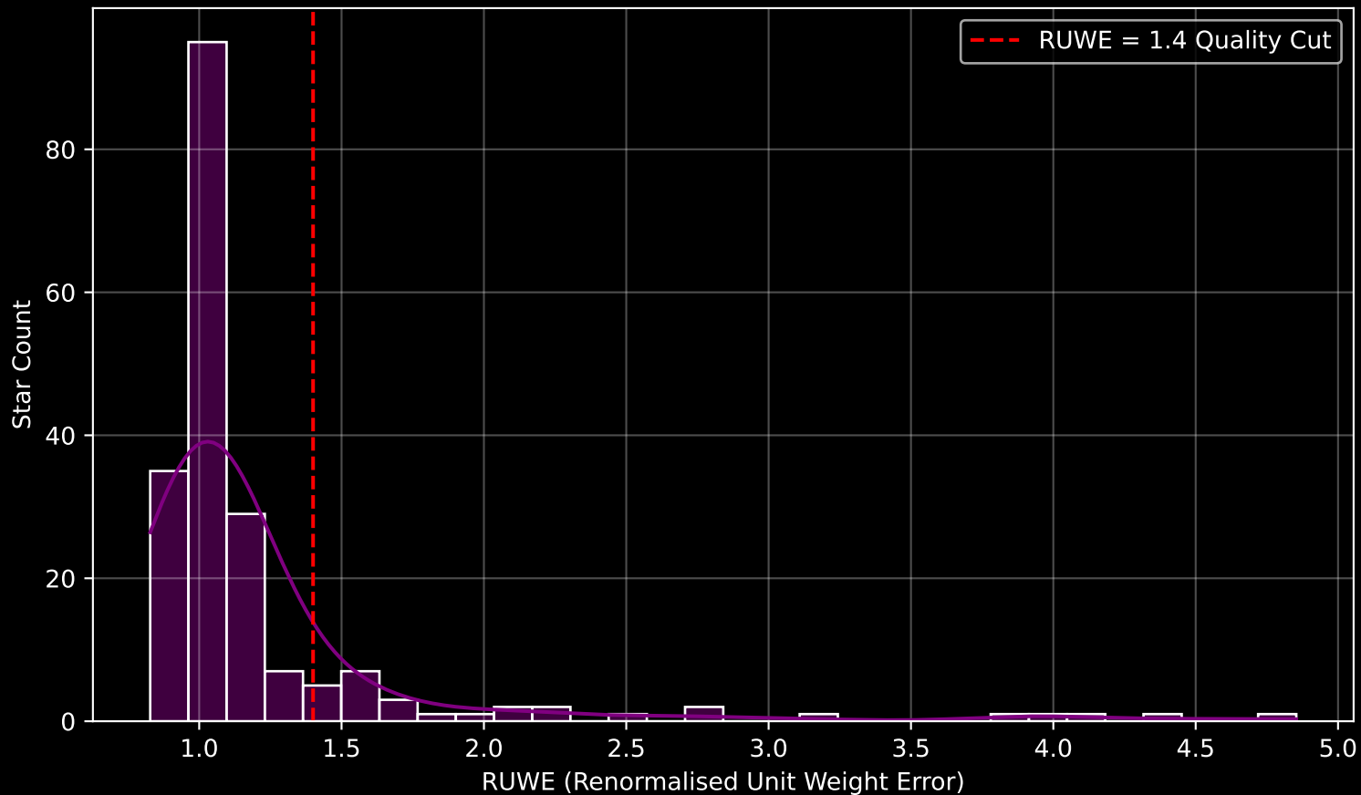
GAPOGEE DR17 Field [K2_C3_043-50] RUWE Distribution (n= 196)
