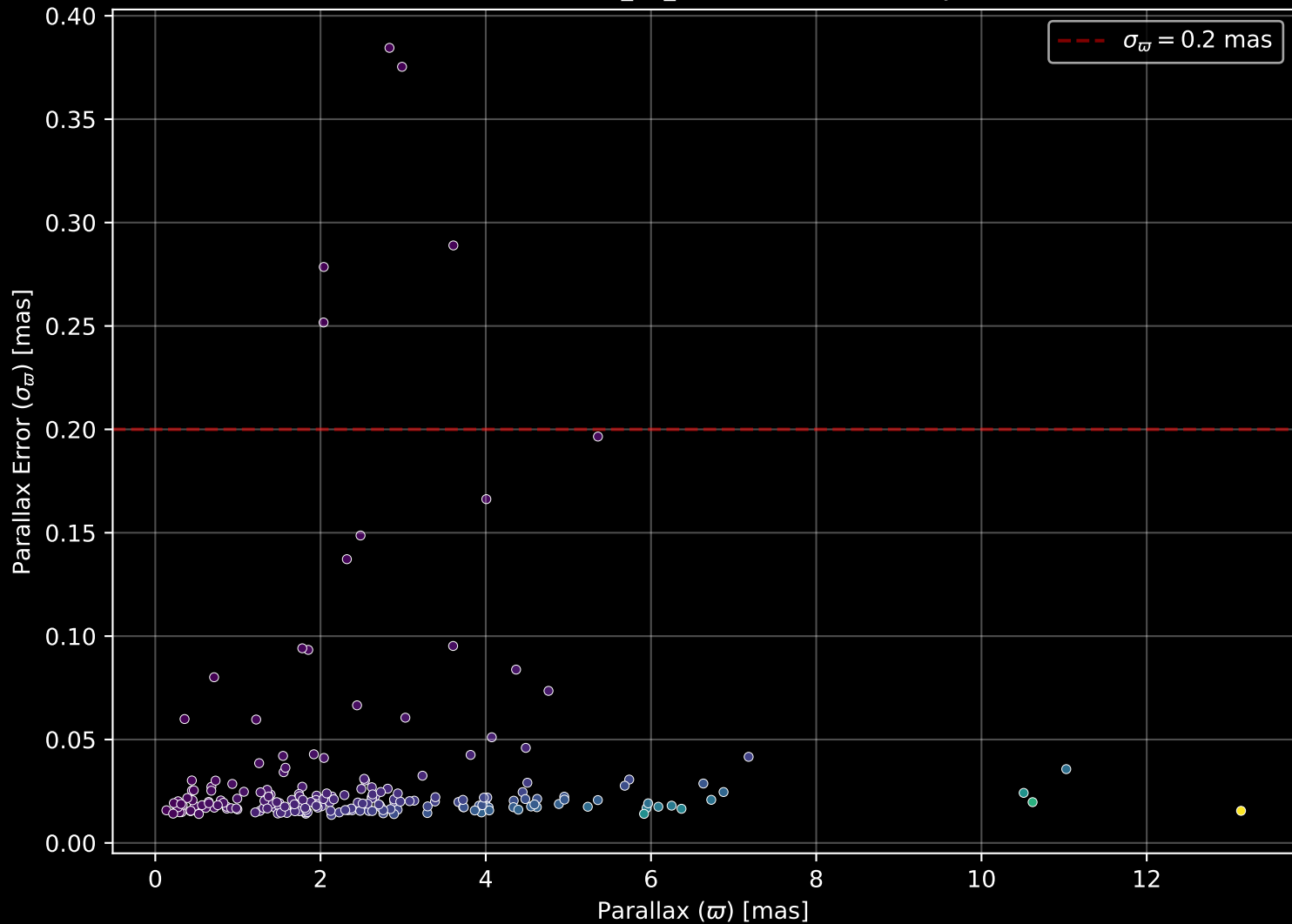
APOGEE DR17 Field: [K2_C3_043-50] Parallax Quality (n= 208)
