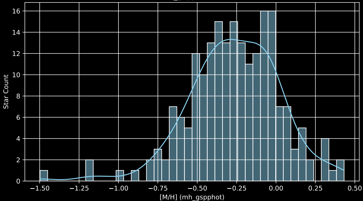
APOGEE DR17 Field: [K2_C3_043-50 [M/H] (mh_gspphot) (n= 207)
