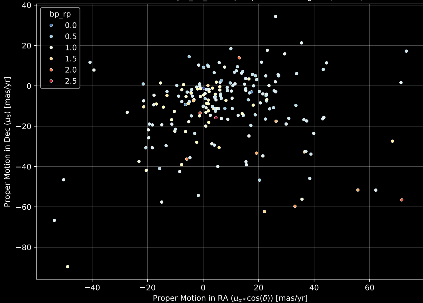
APOGEE DR17 Field: [K2_C3_043-50] Proper Motion Diagram (n= 208)
